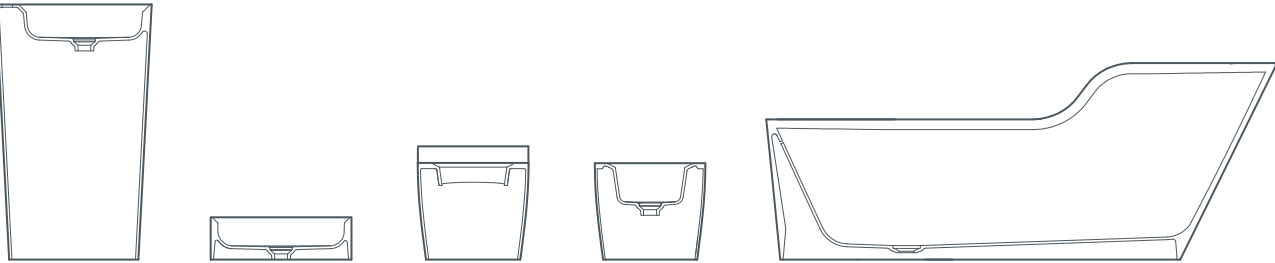
glow washbasin freestanding 55x40x90 cm glow washbasin countertop 50x40x15 cm glow toilet wall hung 52x39x34 cm glow bidet wall hung 52x39x34 cm glow symmetrical bath freestanding 182x84x70/50 cm
